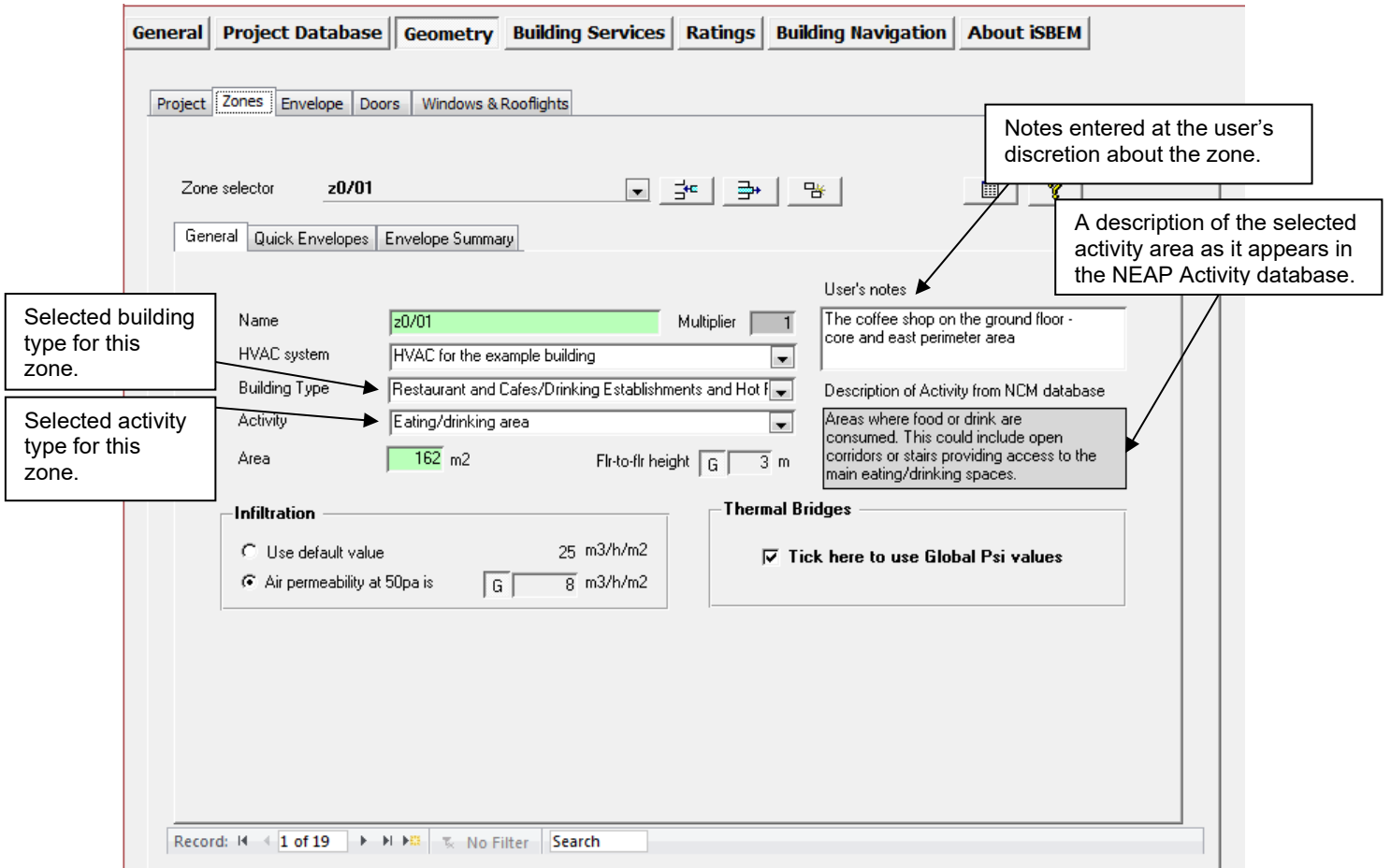
Figure 6: A zone being defined in the General sub-tab of the Zones tab in the Geometry form
