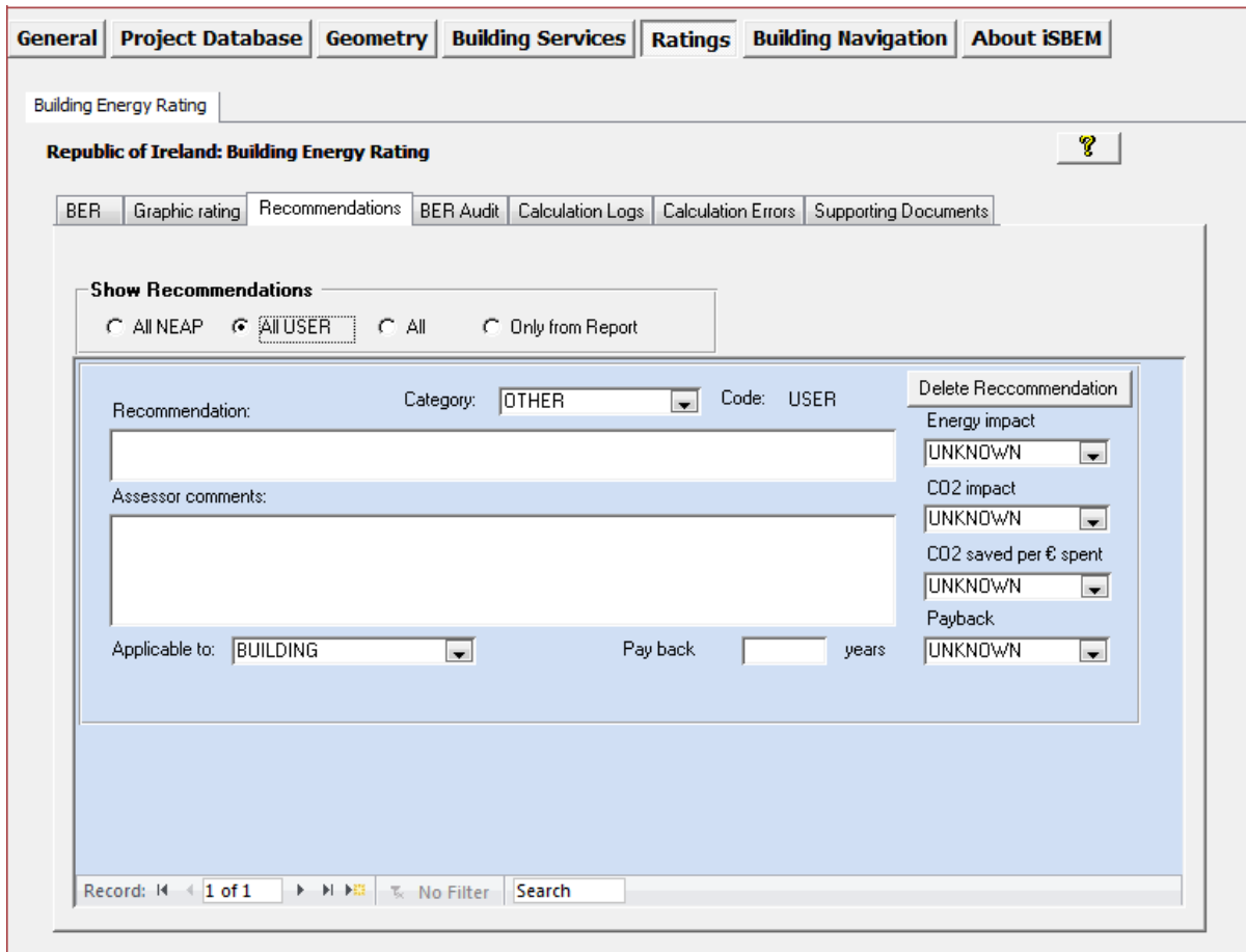
Figure 16: The Recommendations sub-tab in the Building Energy Rating tab of the Ratings form showing the active fields for creating a user-defined recommendation
