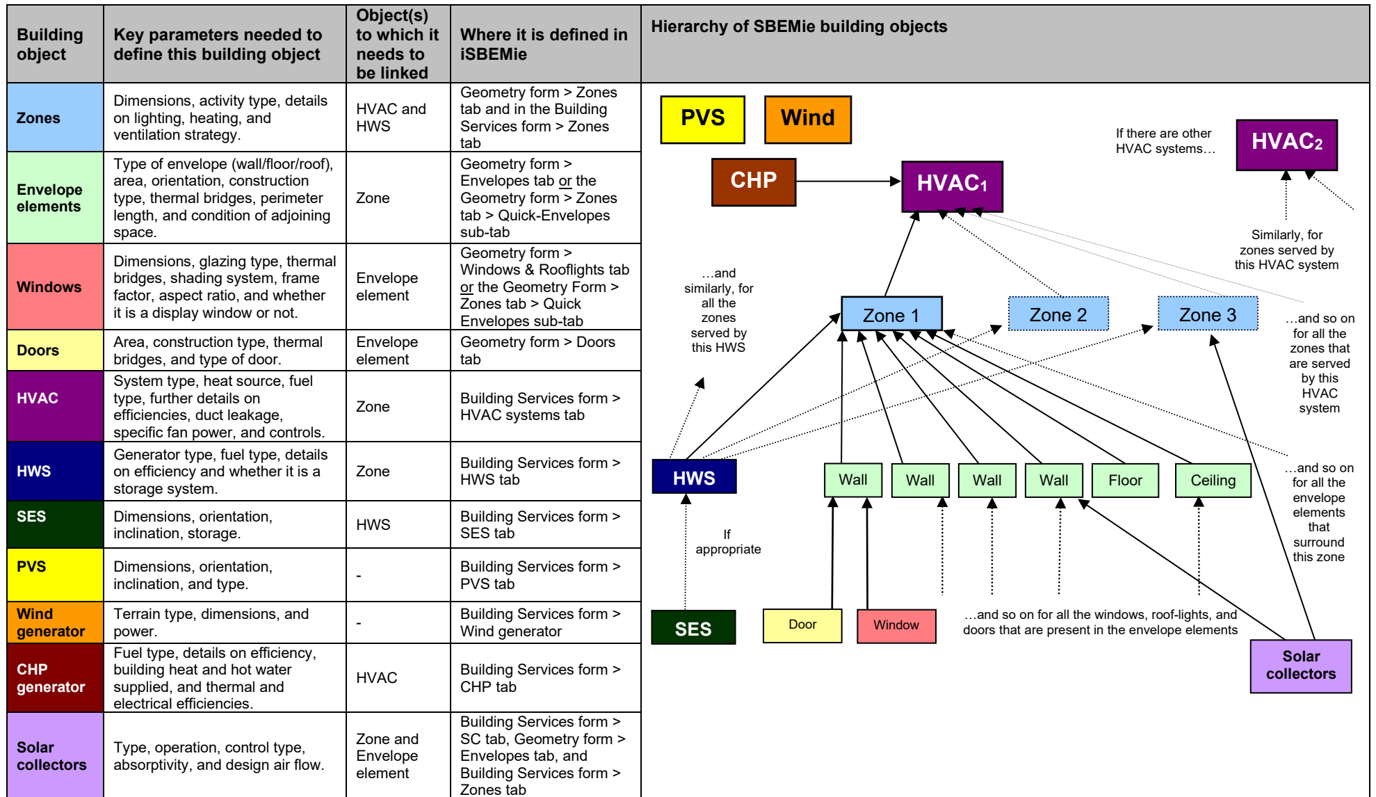
Figure 1: Structure of SBEMie objects
