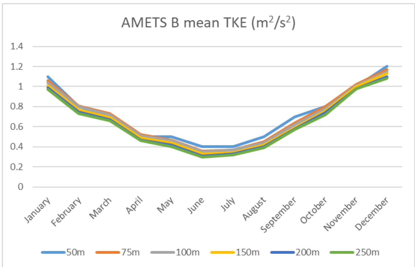
Figure 3. Mean Turbulent Kinetic Energy Summary Graph
