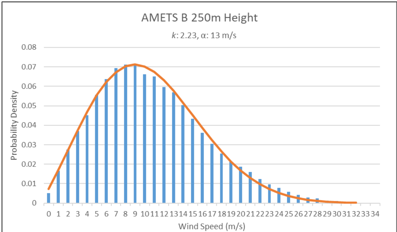
Figure 15. Probability Density Graph for 250m height with Weibull Function in Orange
