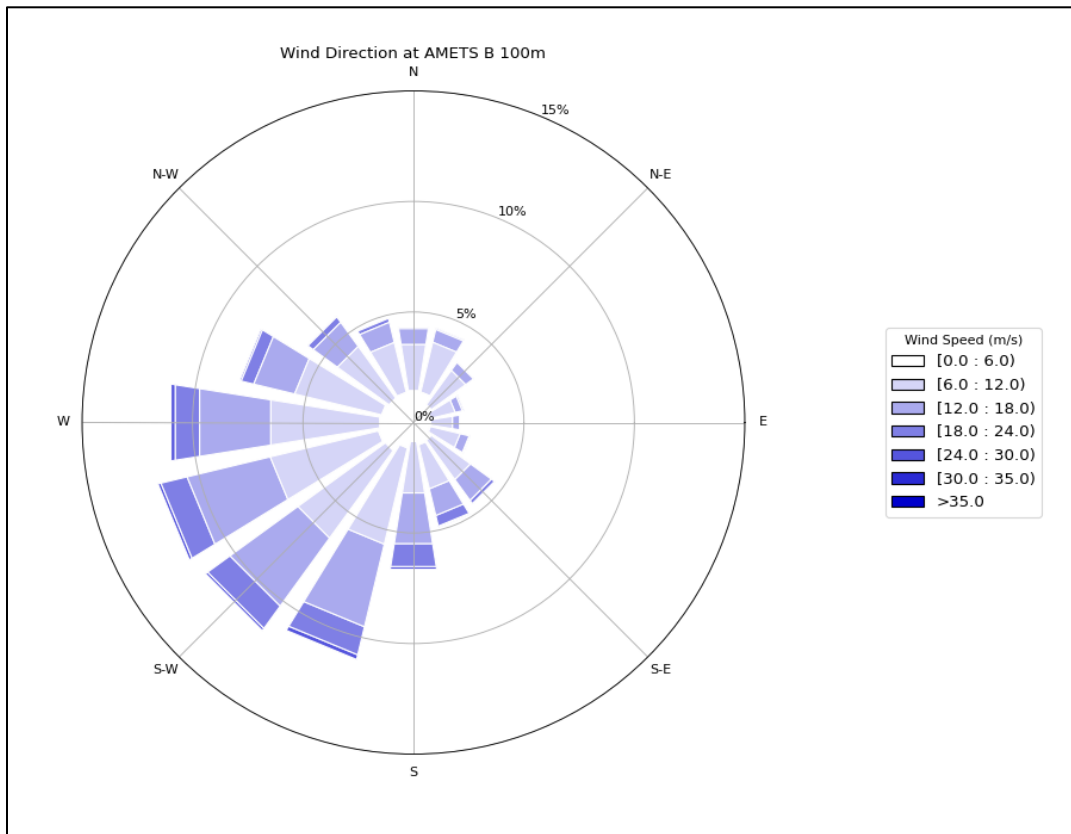
Figure 10. Wind rose showing measured wind direction and wind speed at 100m over the POR
