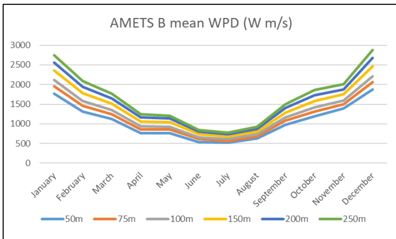
Figure 2. Mean Wind Power Density Summary Graph
