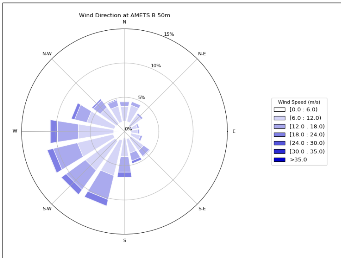
Figure 6. Wind rose showing measured wind direction and wind speed at 50m over the POR
