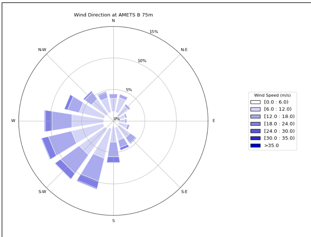
Figure 8. Wind rose showing measured wind direction and wind speed at 75m over the POR
