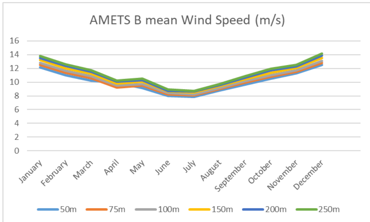
Figure 1. Mean Wind Speed Summary Graph
