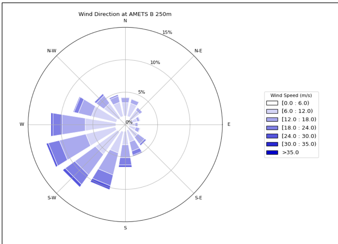
Figure 16. Wind rose showing measured wind direction and wind speed at 250m over the POR
